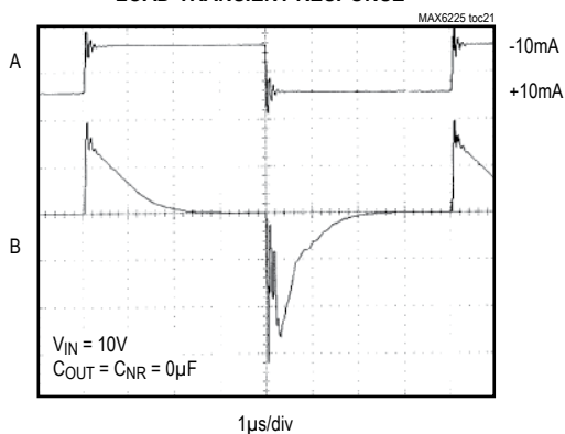
LOAD-TRANSIENT RESPONSE
