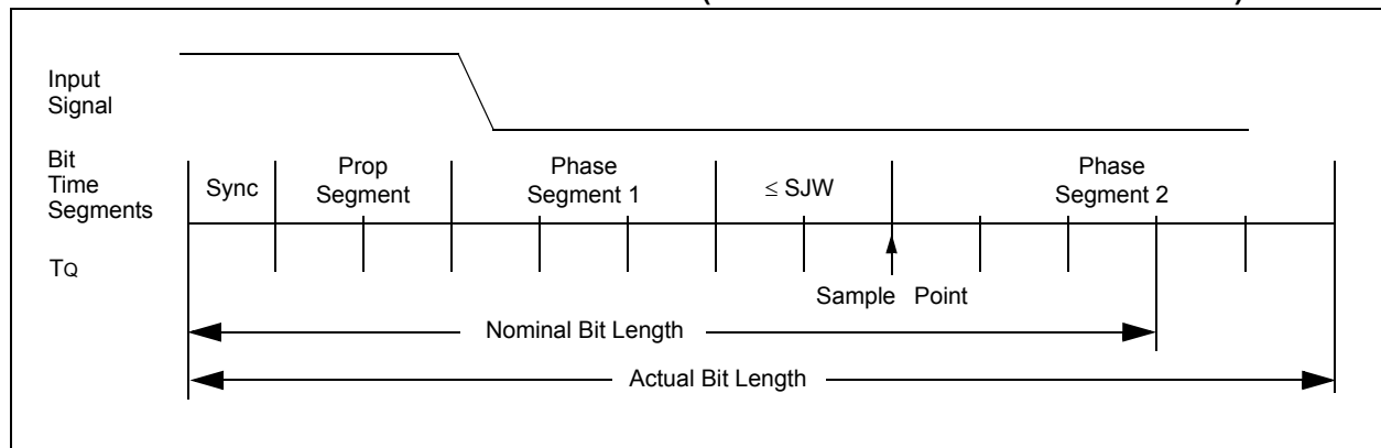
FIGURE 27-6: LENGTHENING A BIT PERIOD (ADDING SJW TO PHASE SEGMENT 1)
