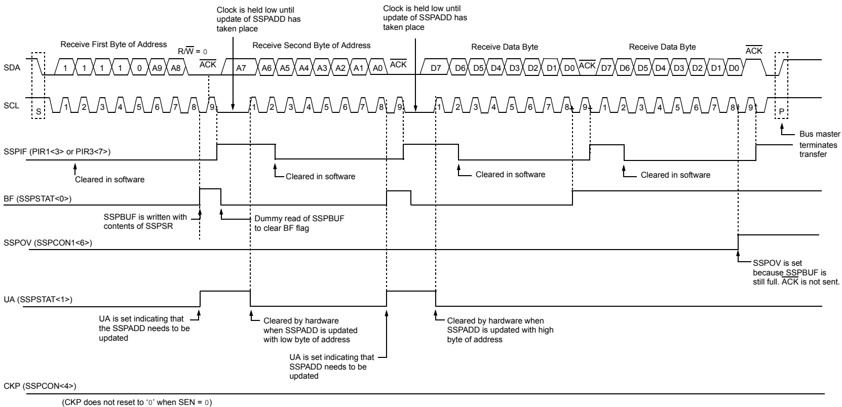
FIGURE 21-12: I 2 C™ SLAVE MODE TIMING WITH SEN = 0 (RECEPTION, 10-BIT ADDRESS)
