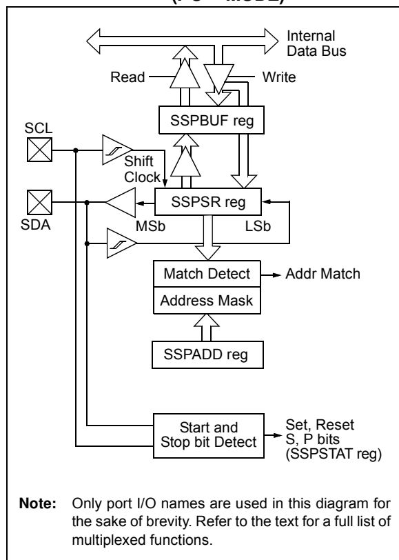
FIGURE 21-7: MSSP BLOCK DIAGRAM (I 2 C™ MODE)
