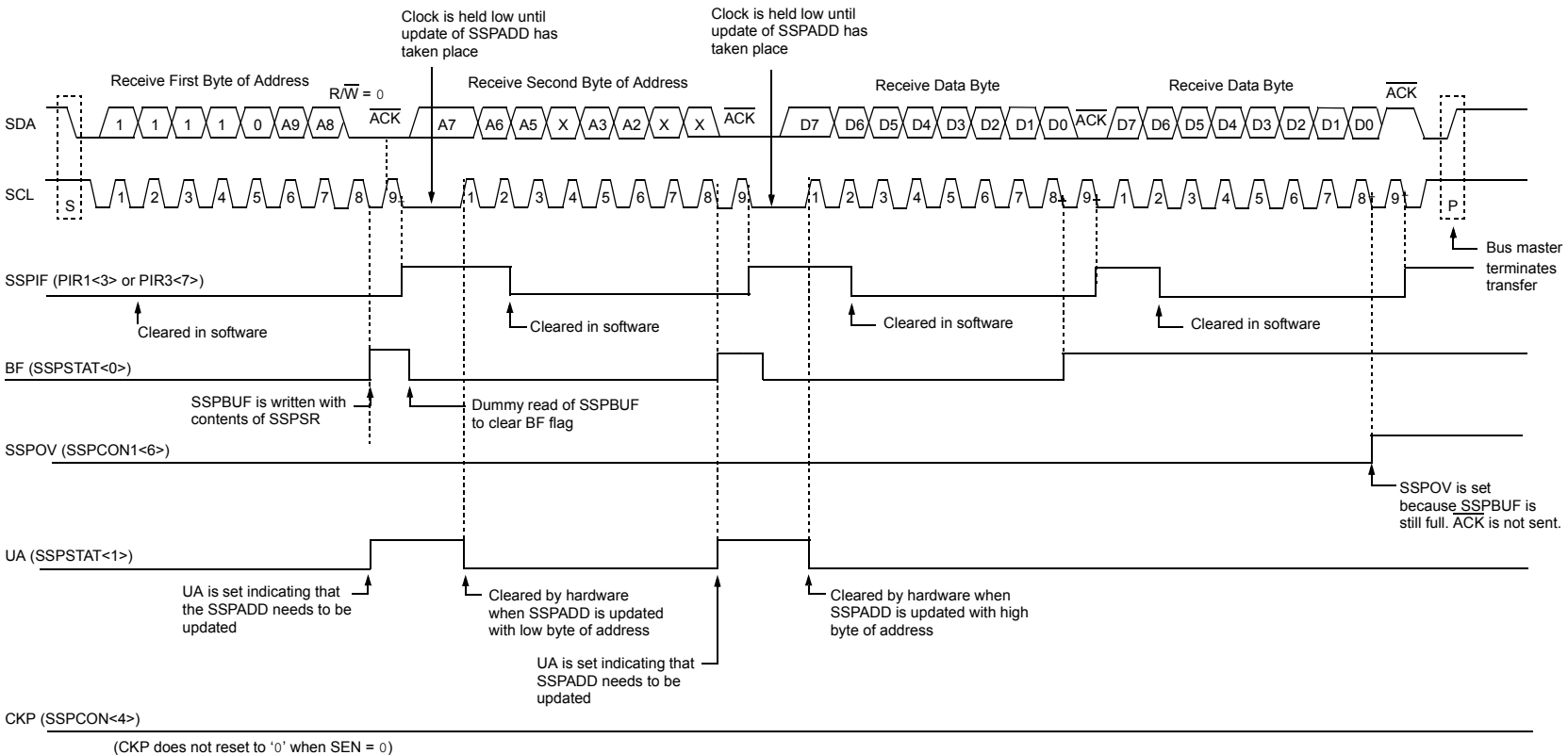
FIGURE 21-11: I 2 C™ SLAVE MODE TIMING WITH SEN = 0 AND ADMSK<5:1> = 01001 (RECEPTION, 10-BIT ADDRESS)
