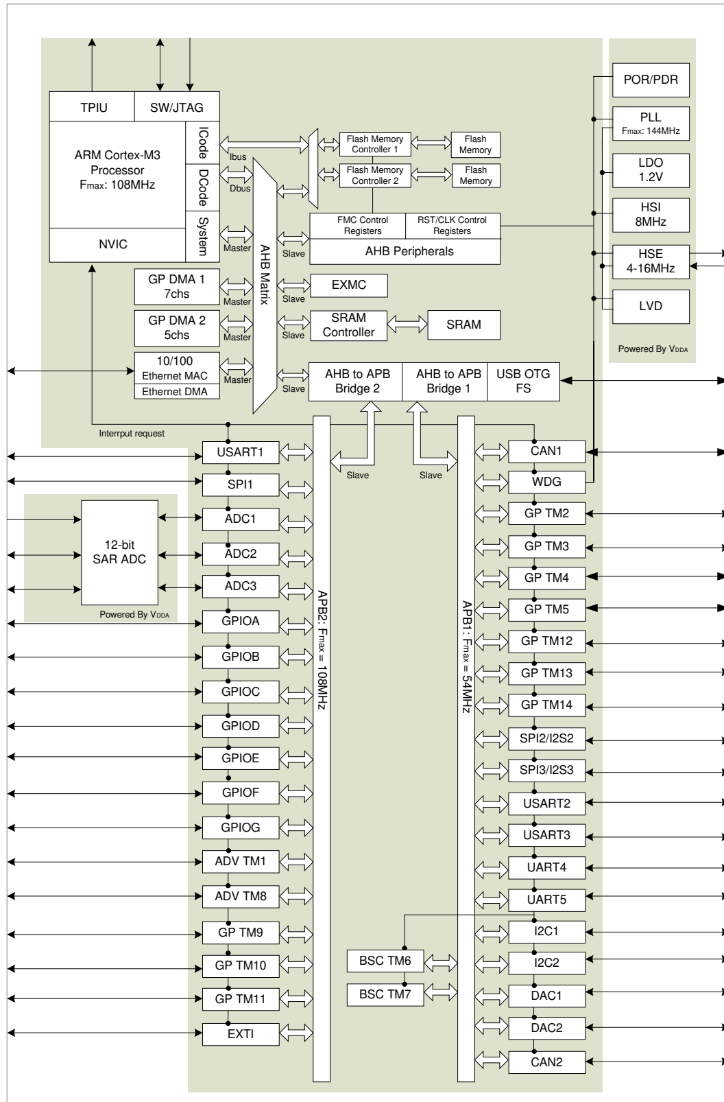
Figure 1. GD32F107xx block diagram
