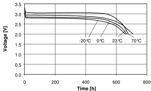
Temperature performance Load 16.2kΩ
