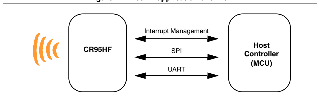
Figure 1. CR95HF application overview
