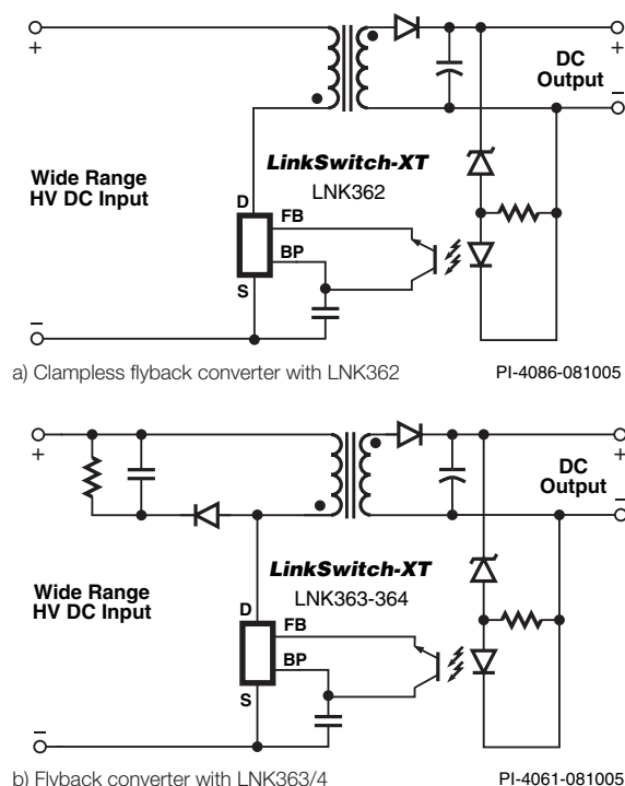
Figure 1. Typical Application with LinkSwitch-XT.
