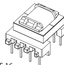
EF 16 reinforced insulation creepage distances: 6mm
