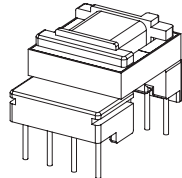
EF 12.6 reinforced insulation creepage distances: 6mm
