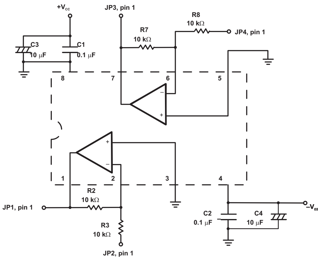
Figure 113. Inverting Amplifiers
