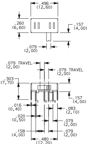
OS203011MA2QP1 DP3T
