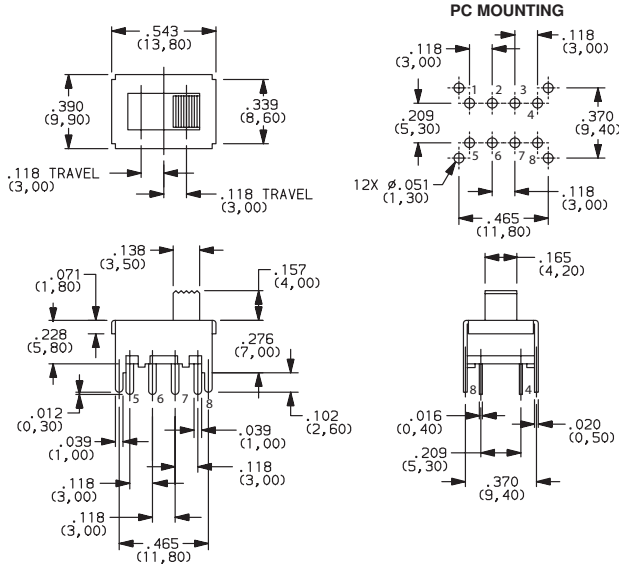
OS203013MT6QN1 DP3T
