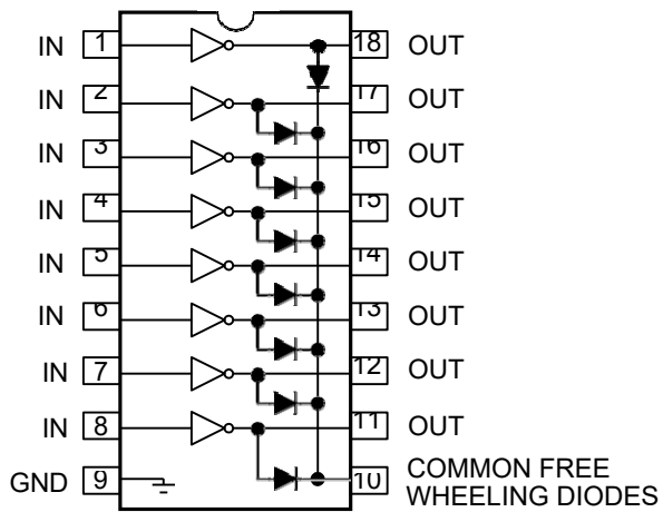
DIP-18/SOP-18
