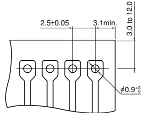
Side entry type
