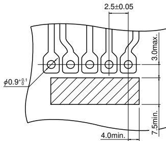
Bottom entry type
