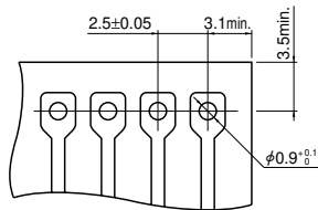
Bottom entry type
