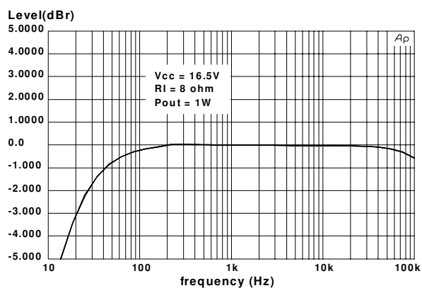
Figure 7: Frequency Response
