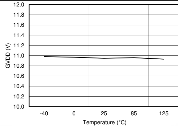
Figure 2. GVDD vs Temperature (PVDD1 = 8 V, EN_GATE = HIGH)
