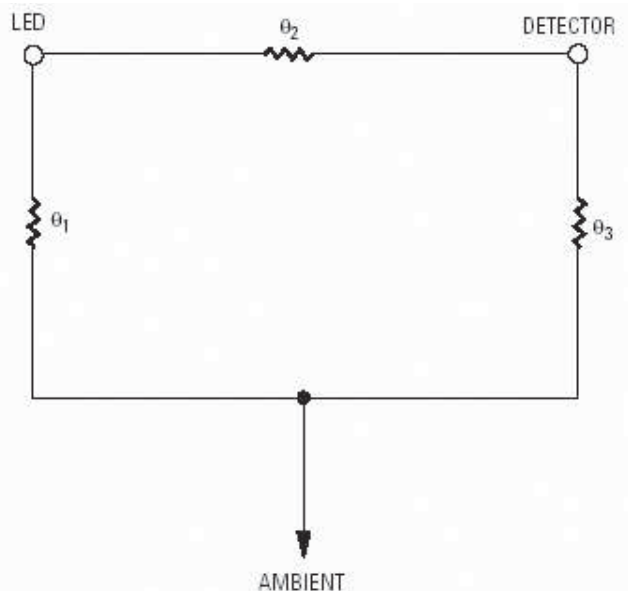
Figure 29. Thermal Model-B Diagram
