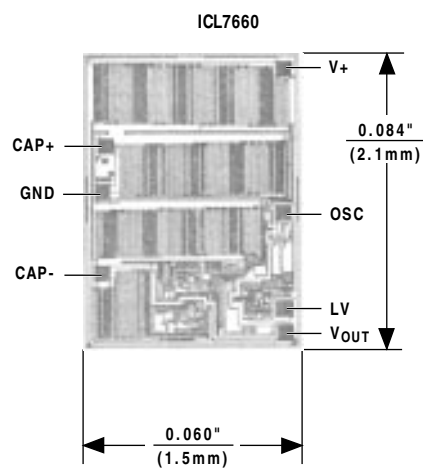
TRANSISTOR COUNT: 71 SUBSTRATE CONNECTED TO V+
