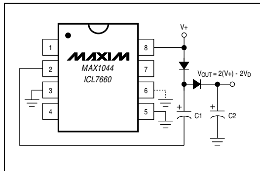
Figure 9. Voltage Doubler
