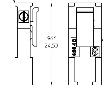
MATED MICRO-FIT CONNECTOR
