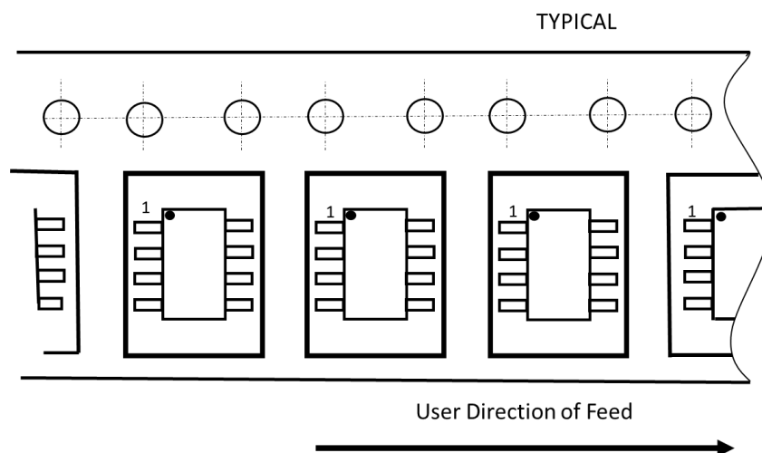
Figure 23. Tape orientation
