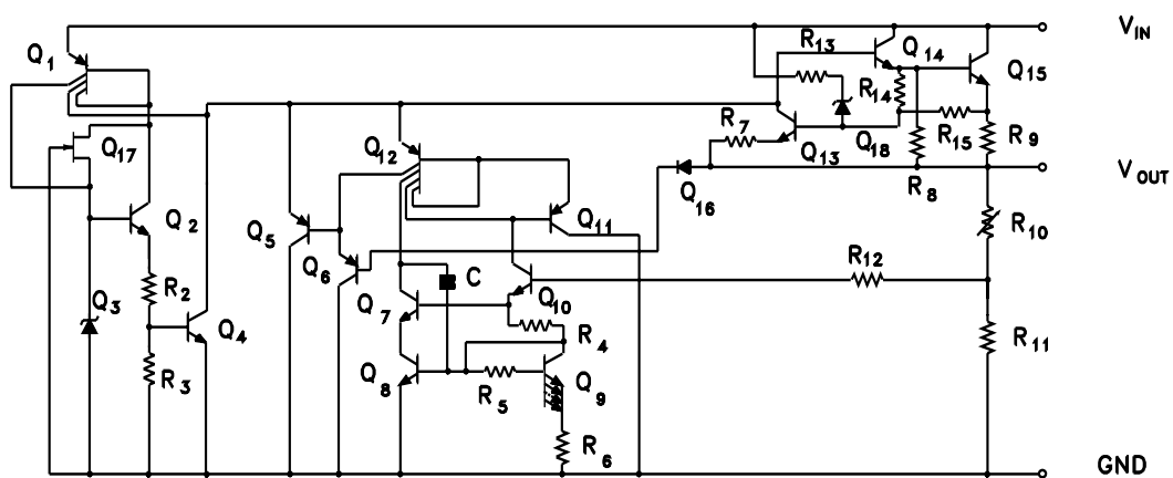
Figure 1. Schematic diagram
