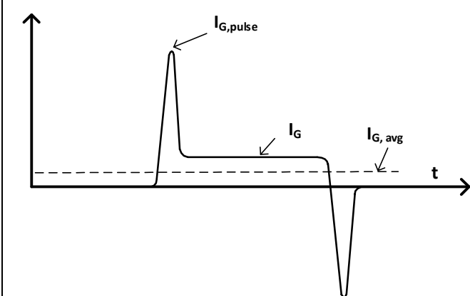
Figure 27 Gate current switching waveform
