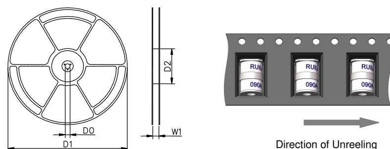
Direction of Unreeling
