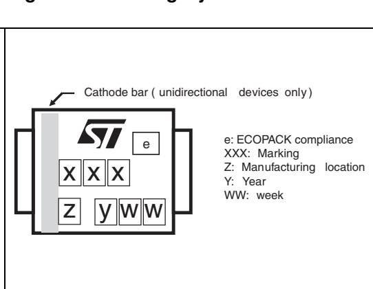
Figure 14. Marking layout (1)
