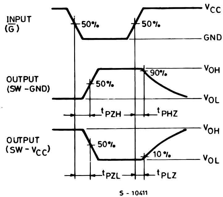
WAVEFORM 2: OUTPUT ENABLE AND DISABLE TIMES ( f=1\text{MHz} ; 50% duty cycle)
