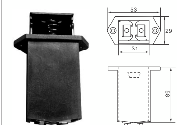
SBH-9V-COM FOR ONE "9V" CELL (NEW)
