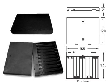
SBH-3201S/MV FOR TWENTY "AA" CELLS
