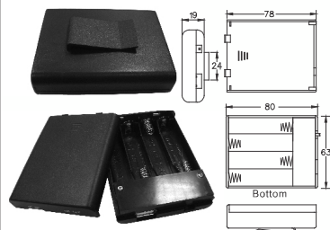
SBH-341-3A FOR FOUR "AA" CELLS SBH-341-3AS SBH-341-3S/USB
