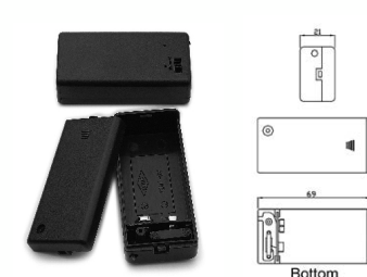
SBH-9VA FOR ONE "9V" CELL SBH-9VAS SBH-9VP
