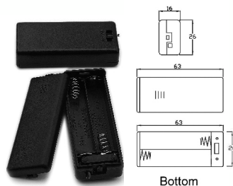
SBH-421-1A FORTWO "AAA" CELLS SBH-421-1AS
