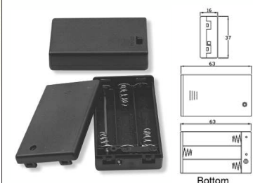
SBH-431-1A FOR THREE "AAA" CELLS SBH-431-1AS
