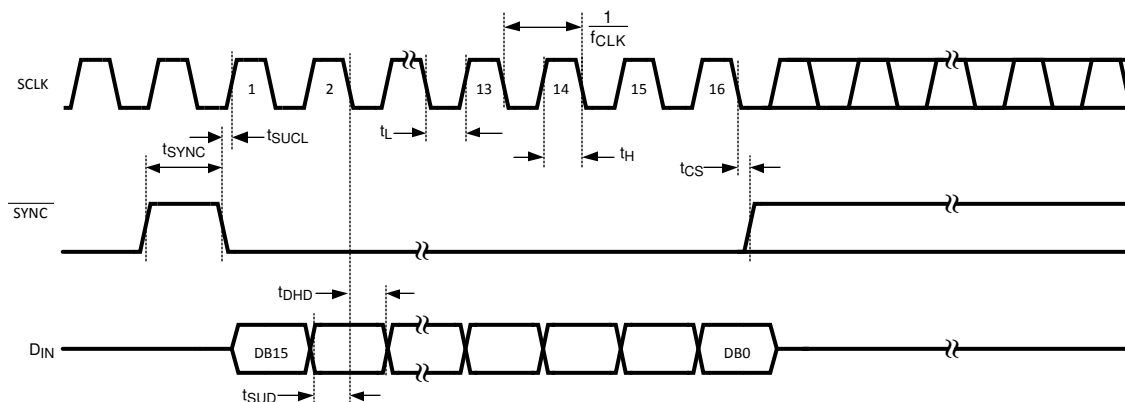
Figure 2. DAC081S101 Timing
