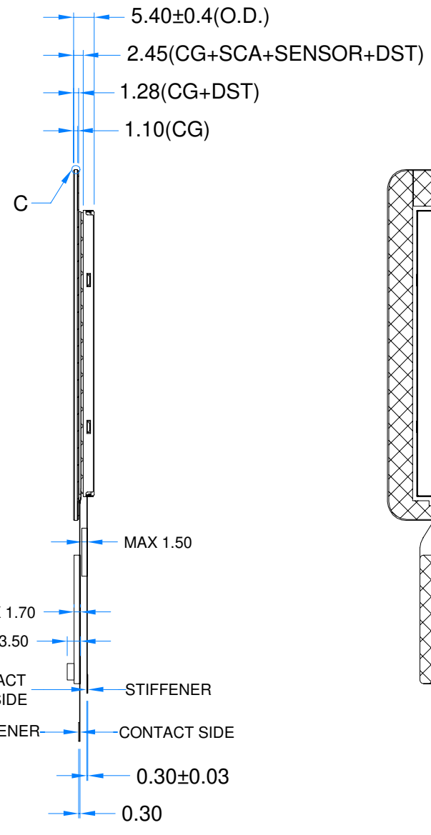
DETAIL C SCALE 4:1
