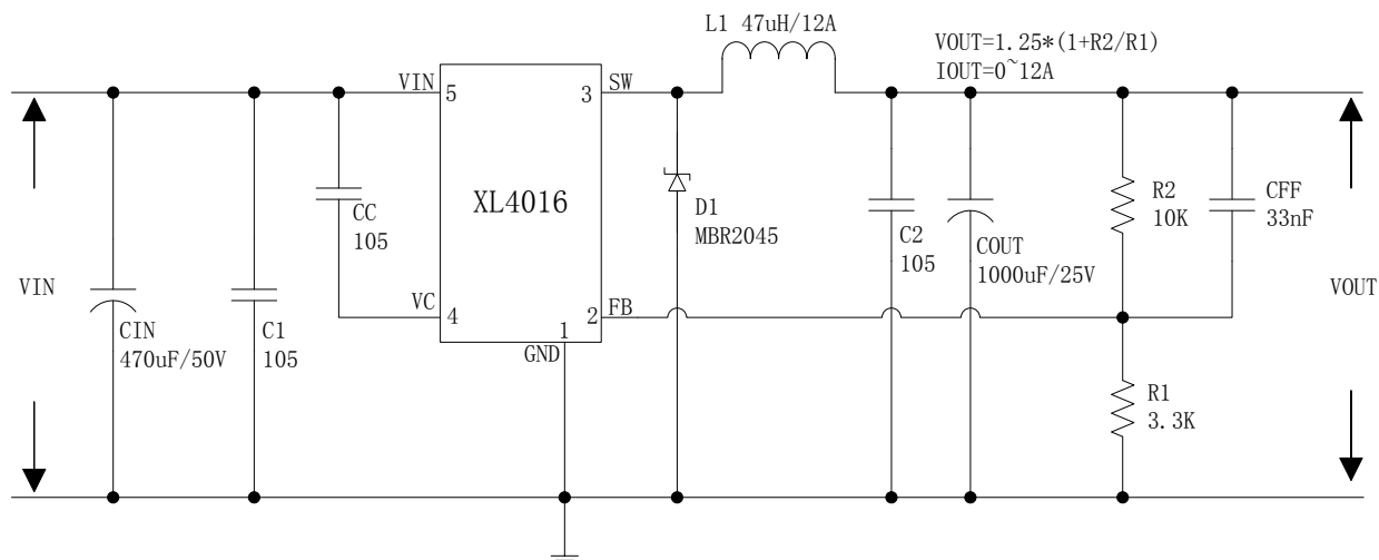
Figure5. XL4016 System Parameters Test Circuit ( V_{IN}=8V\sim 36V , V_{OUT}=5V/12A )
