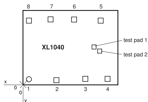
Fig.9 Bonding pad locations.
