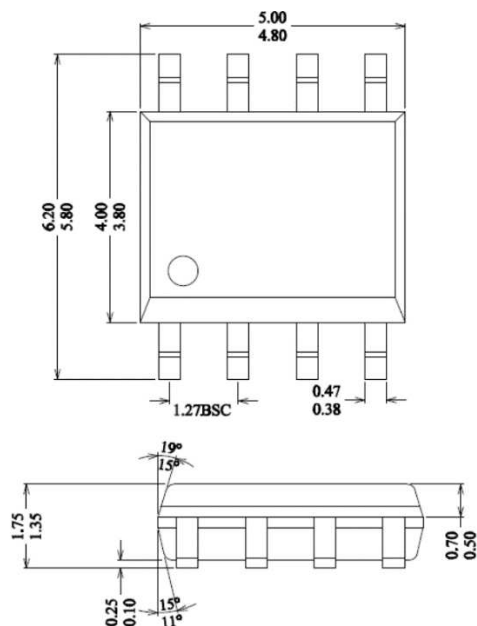
Figure19. 8-Lead Standard Small Outline Package [8-Lead SOIC_N]
