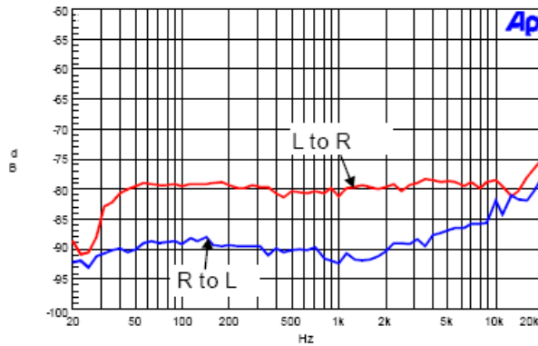
14. Crosstalk
