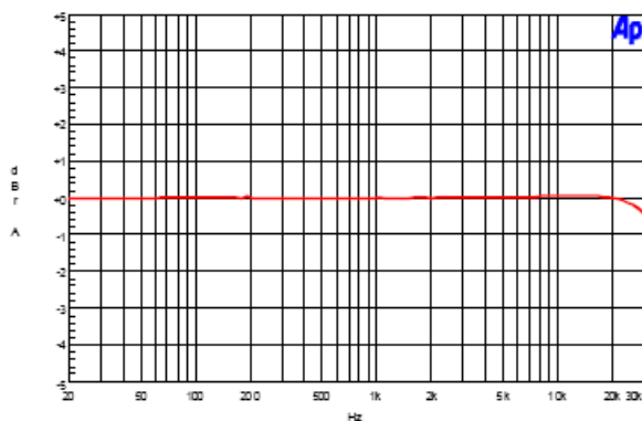
15. Frequency Response ( V_o = 1.0\text{V}_{rms} )
