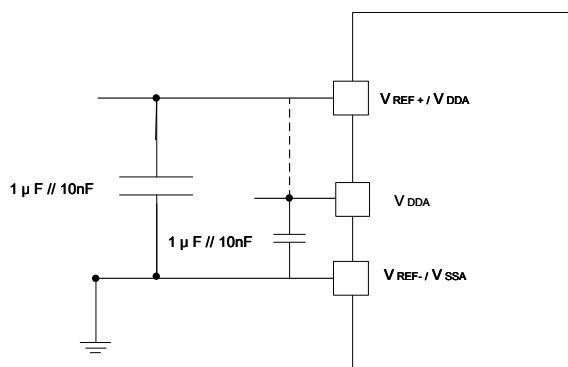
Map 25 Power supply and the reference power supply decoupling circuit ( V_{REF+} Not with V_{DD+} Connected)
