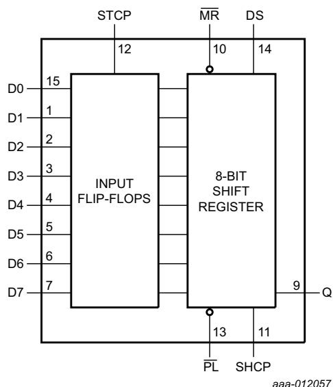
Fig 1. Functional diagram
