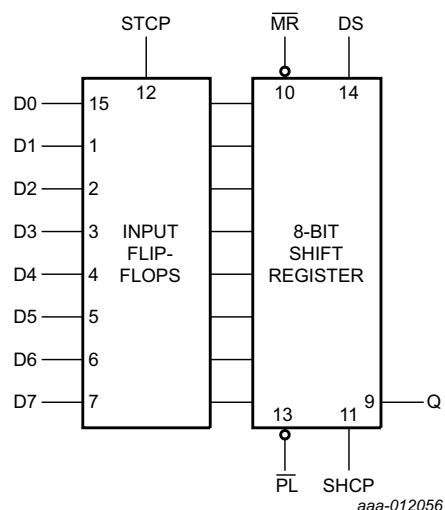
Fig 2. Logic symbol
