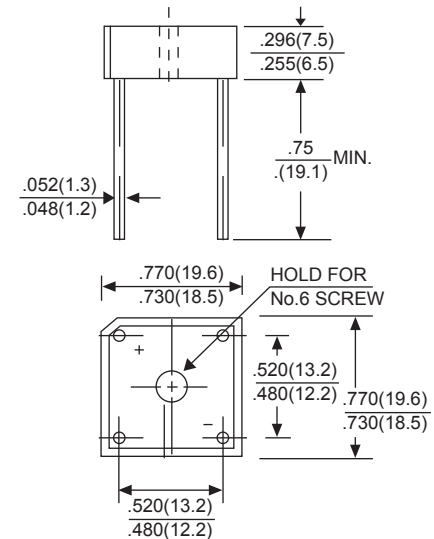
KBPC/8-10
