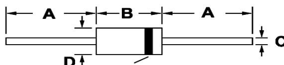
DO-201AD Axial Leaded Plastic Package
