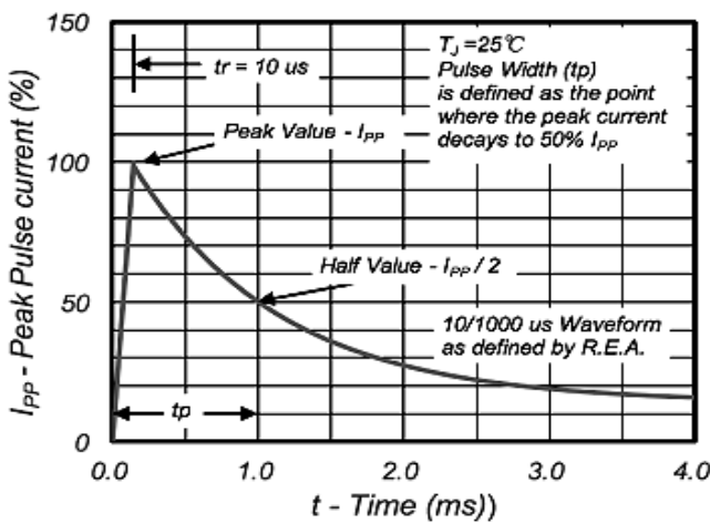
Fig 2: Pulse Waveform
