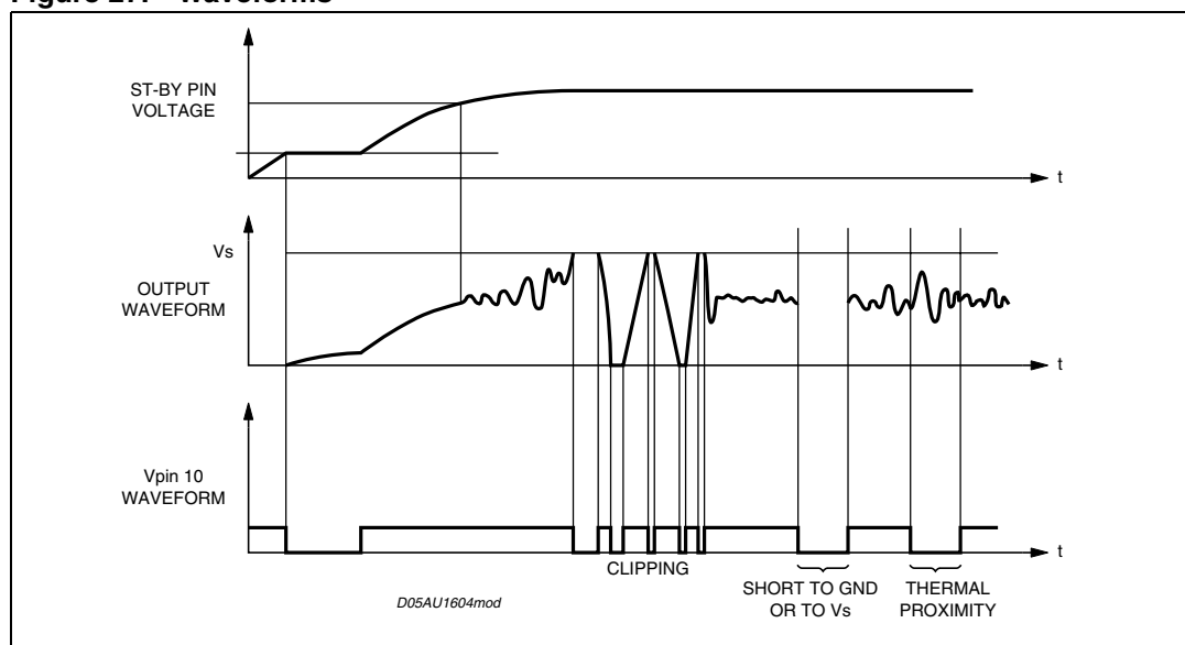
Figure 27. Waveforms
