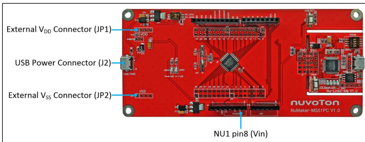
Figure 2.5-2 External Power Supply Sources on MS51 Platform
