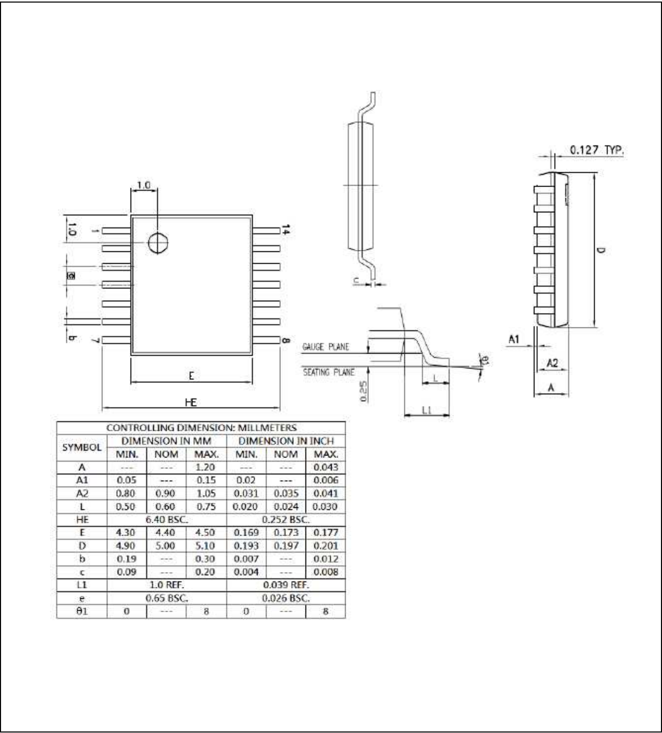
Figure 9.1-1 TSSOP-14 Package Dimension
