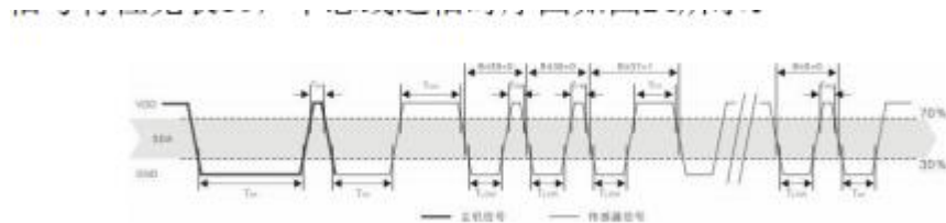
Figure 24: AM2305B Single Bus Communication Timing
