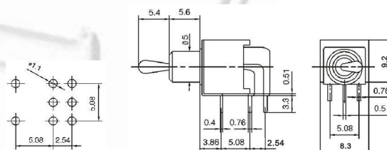
TSSM2022C3 ON-ON TSSM2032C3 ON-OFF-ON DPDT 6P
