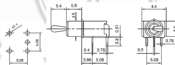
TSSM1022C3 ON-ON TSSM1032C3 ON-OFF-ON SPDT 3P
