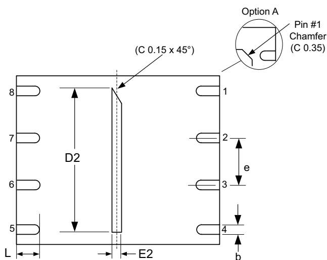
BOTTOM VIEW
