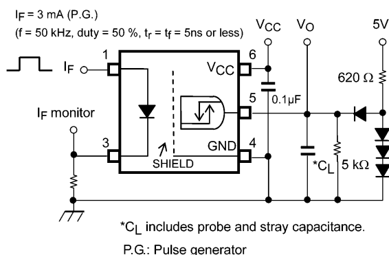
Fig. 12.1.7 Switching Time Test Circuit and
