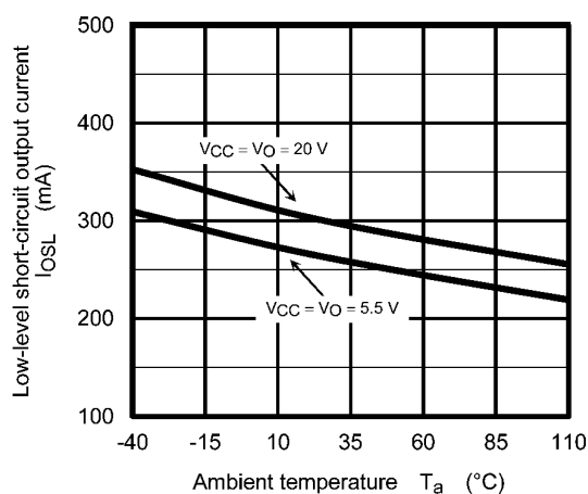
Fig. 12.2.9 I_{osL} - T_a
