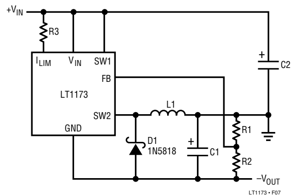
Figure 7. Positive-to-Negative Converter
