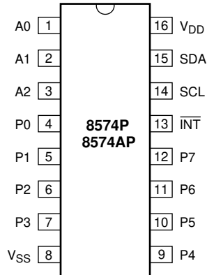
Fig 3. Pin configuration for DIP16
