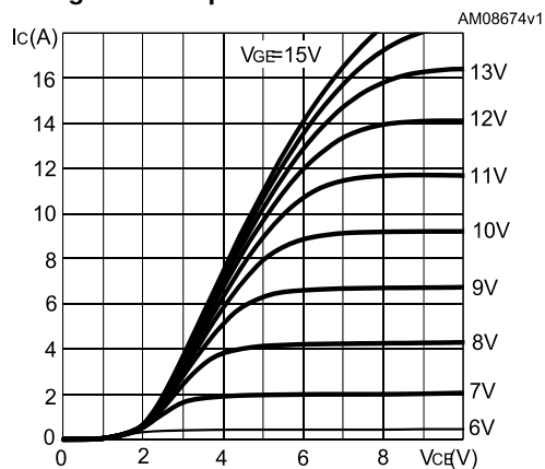
Figure 2: Output characteristics
