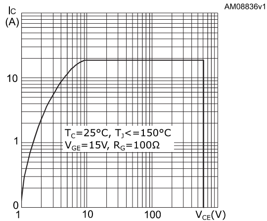
Figure 14: Turn-off SOA
