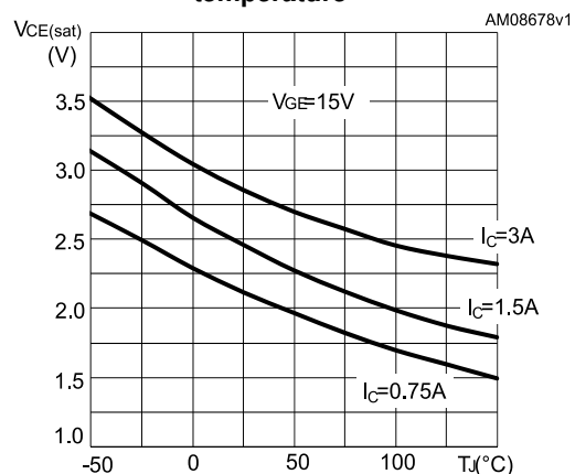
Figure 6: Collector-emitter on voltage vs temperature
