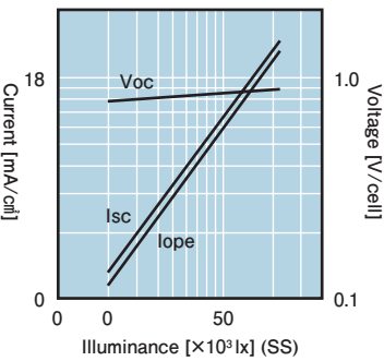
Relationship between Output and Illuminance
