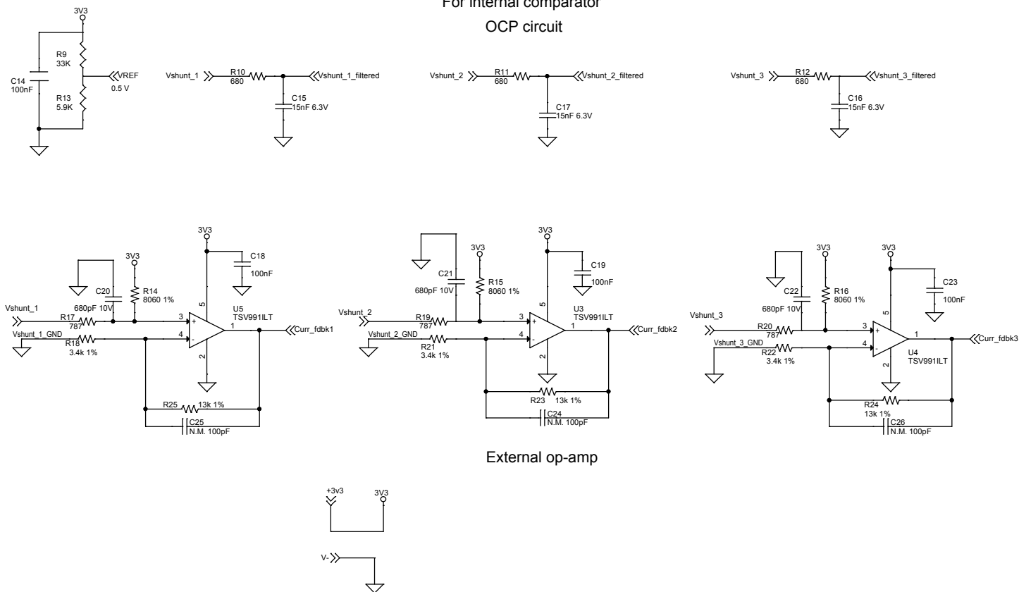
Figure 3. STEVAL-ESC001V1 circuit schematic (3 of 4)
