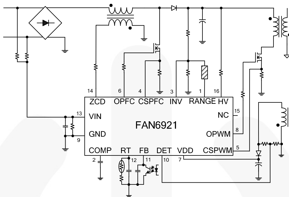
Figure 1. Typical Application
