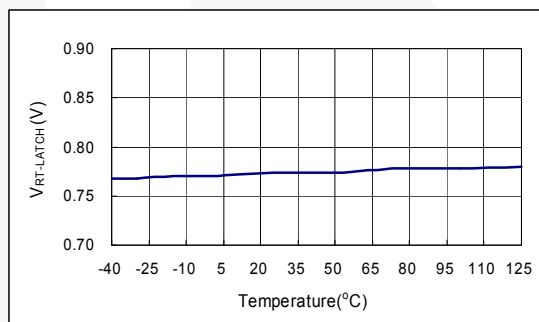
Figure 24. Over Temperature Protection Threshold Voltage of RT Pin
