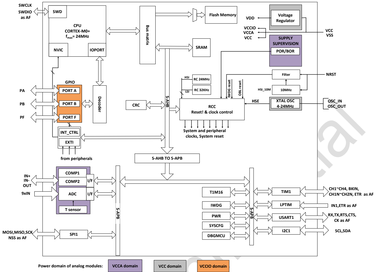
Figure 1-1 Functional Module
