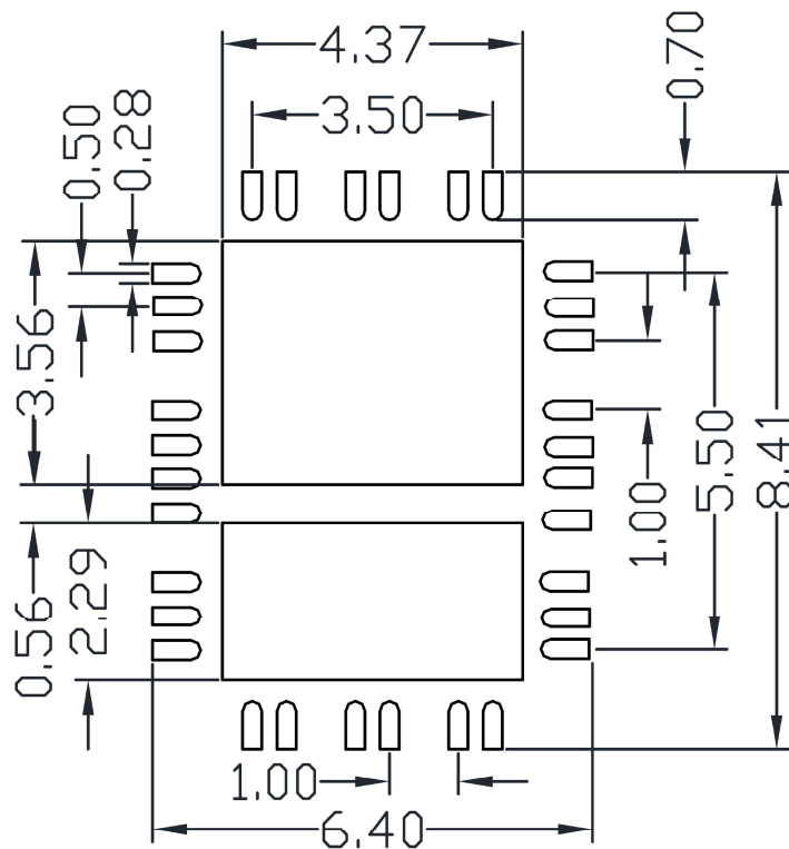
Figure 7 • PD70224 Top layer Copper Recommended PCB Layout (mm)
