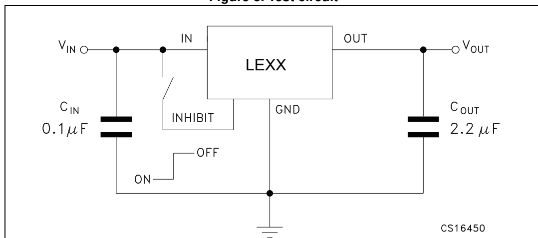
Figure 3. Test circuit
