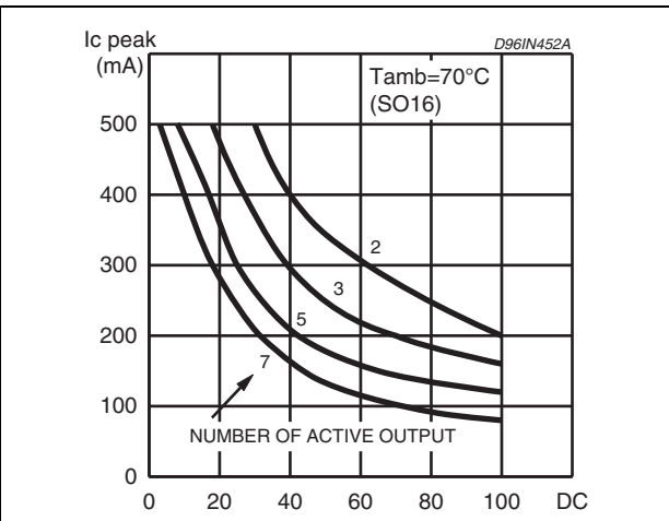
Figure 16. Peak collector current vs. duty cycle (SO-16)
